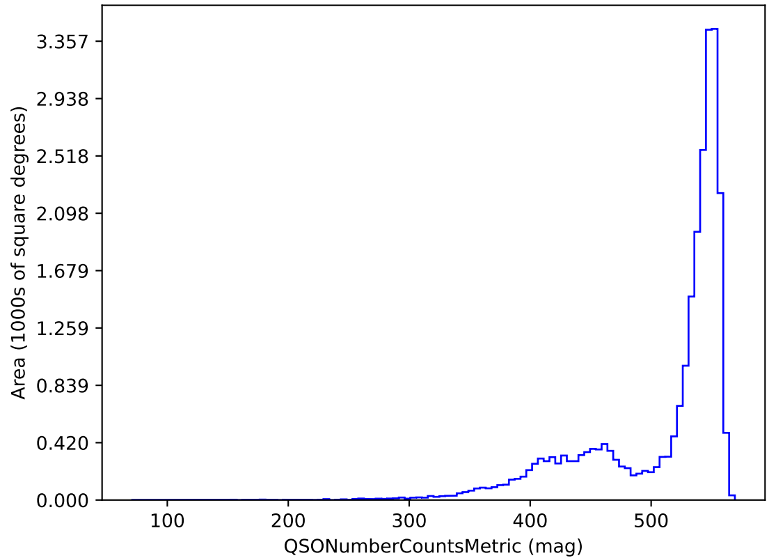
weather_cloudso10v3.4_10yrs i band and non-DD: QSONumberCountsMetric
