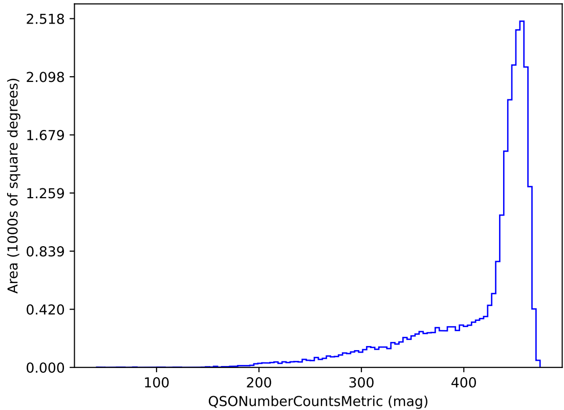
weather_cloudso10v3.4_10yrs g band and non-DD: QSONumberCountsMetric
