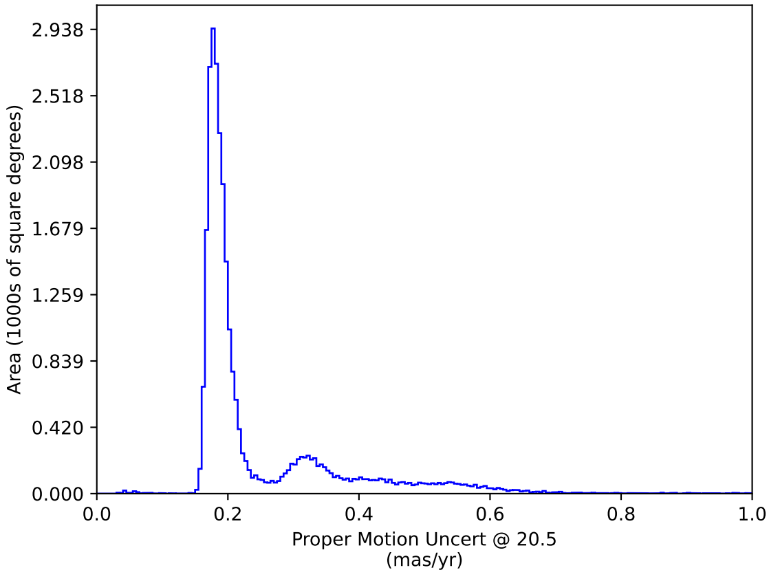
weather_cloudso10v3.4_10yrs : Proper Motion Uncert @ 20.5
