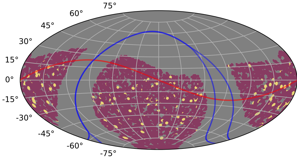
weather_cloudso10v3.4_10yrs : PrestoKNe_score_s
