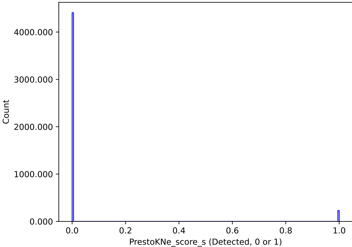
weather_cloudso10v3.4_10yrs : PrestoKNe_score_s
