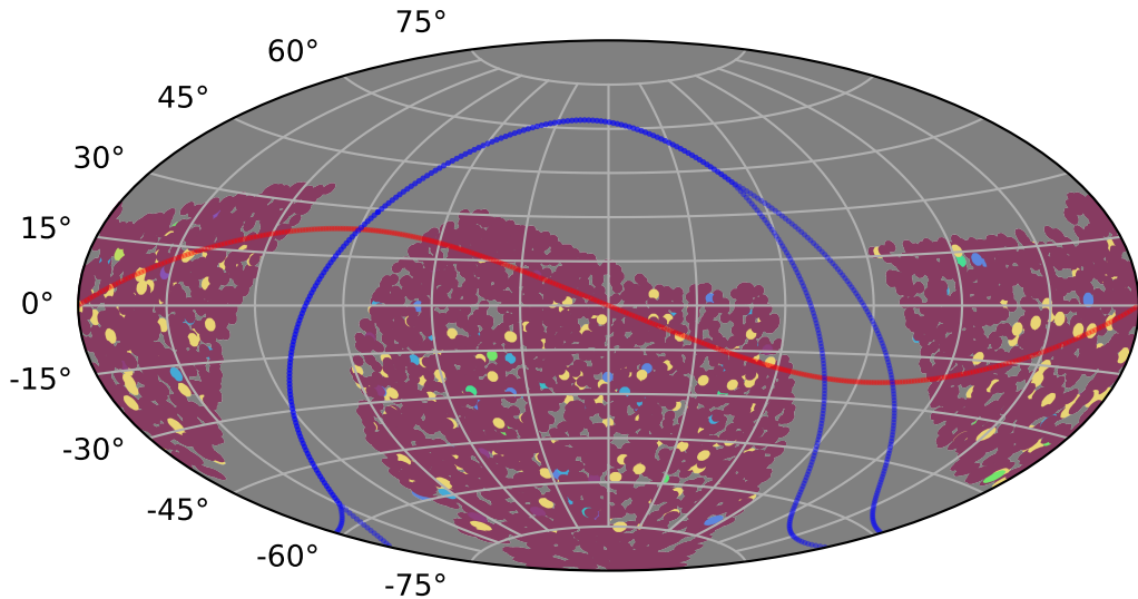
weather_cloudso10v3.4_10yrs : PrestoKNe_score_p
