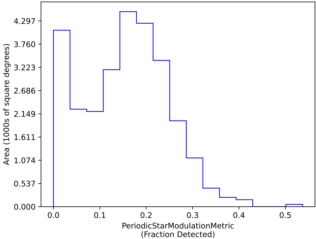
weather_cloudso10v3.4_10yrs dm 20 interval 30 RRC Year 1-2: PeriodicStarModulationMetric
