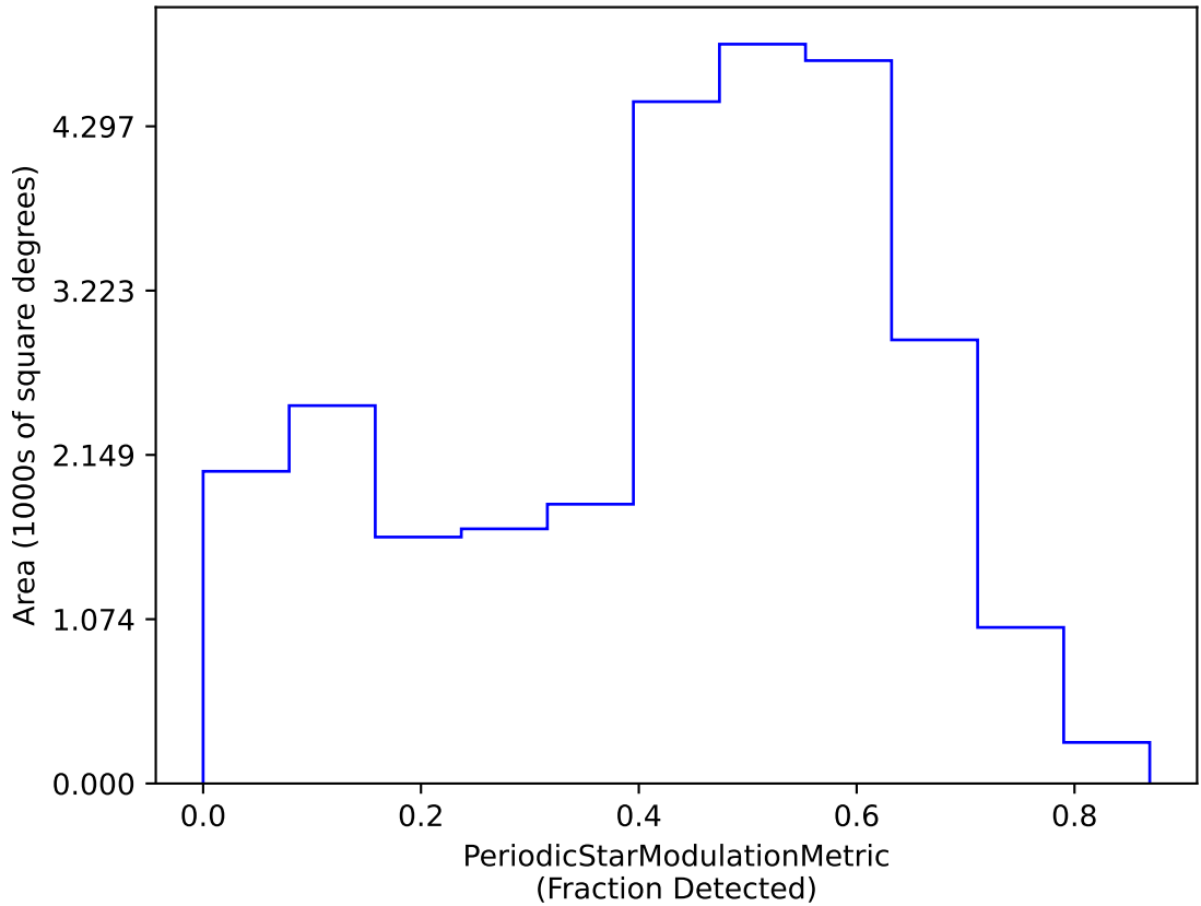
weather_cloudso10v3.4_10yrs dm 18 interval 30 RRC Year 1-2: PeriodicStarModulationMetric
