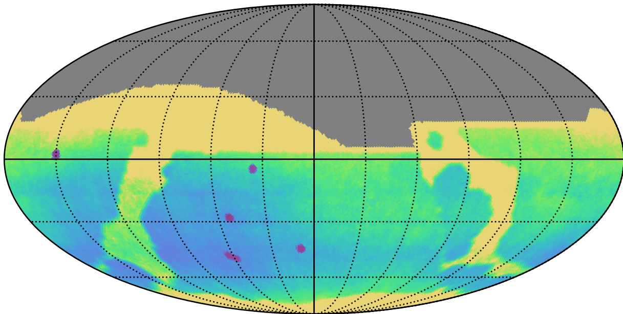
weather_cloudso10v3.4_10yrs : Parallax Uncert @ 24.0
