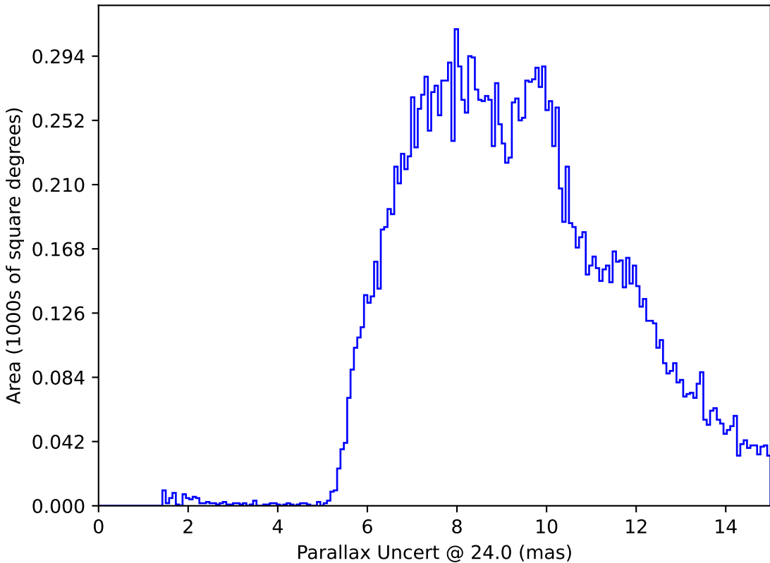
weather_cloudso10v3.4_10yrs : Parallax Uncert @ 24.0
