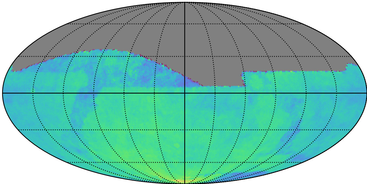
weather_cloudso10v3.4_10yrs : Parallax Coverage @ 22.4
