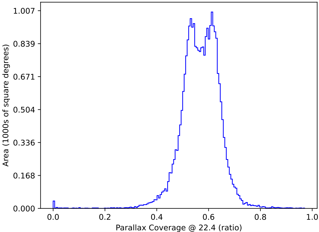
weather_cloudso10v3.4_10yrs : Parallax Coverage @ 22.4
