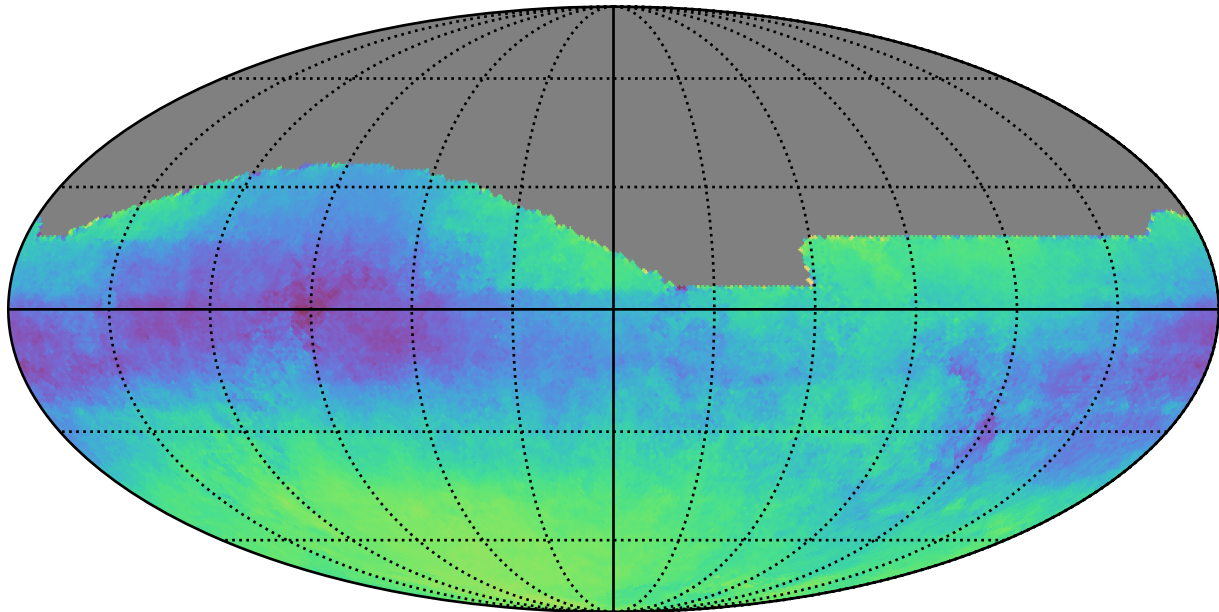
weather_cloudso10v3.4_10yrs : Parallax-DCR degeneracy @ 24.0
