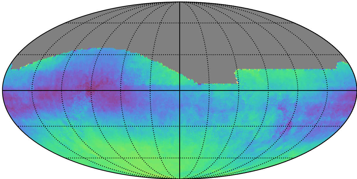
weather_cloudso10v3.4_10yrs : Parallax-DCR degeneracy @ 22.4
