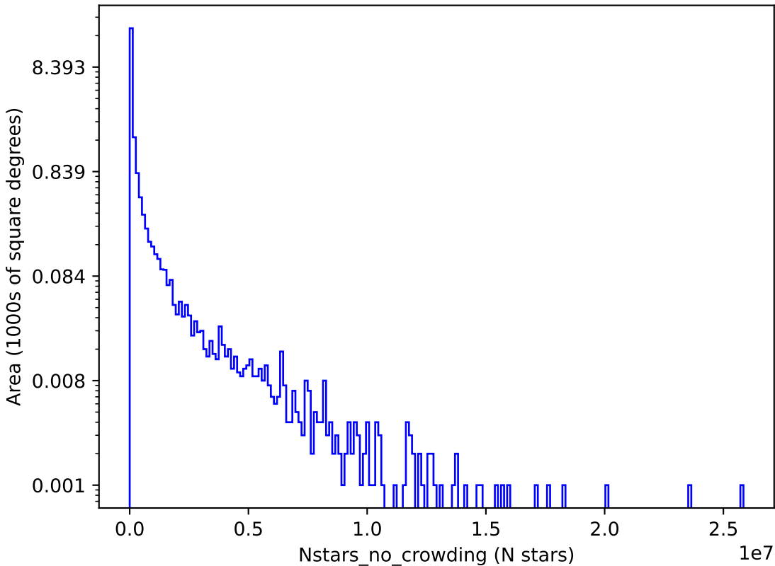
weather_cloudso10v3.4_10yrs y: Nstars_no_crowding
