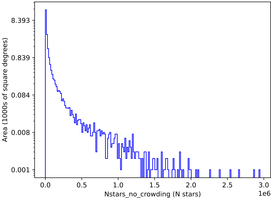
weather_cloudso10v3.4_10yrs u: Nstars_no_crowding
