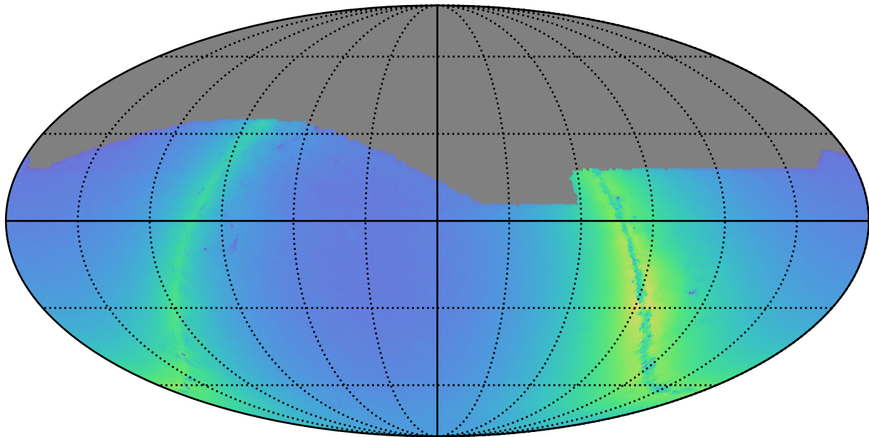
weather_cloudso10v3.4_10yrs r: Nstars_no_crowding
