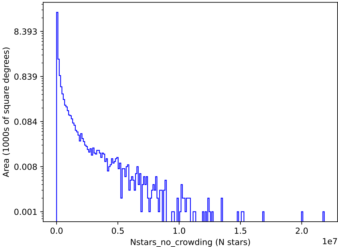
weather_cloudso10v3.4_10yrs r: Nstars_no_crowding
