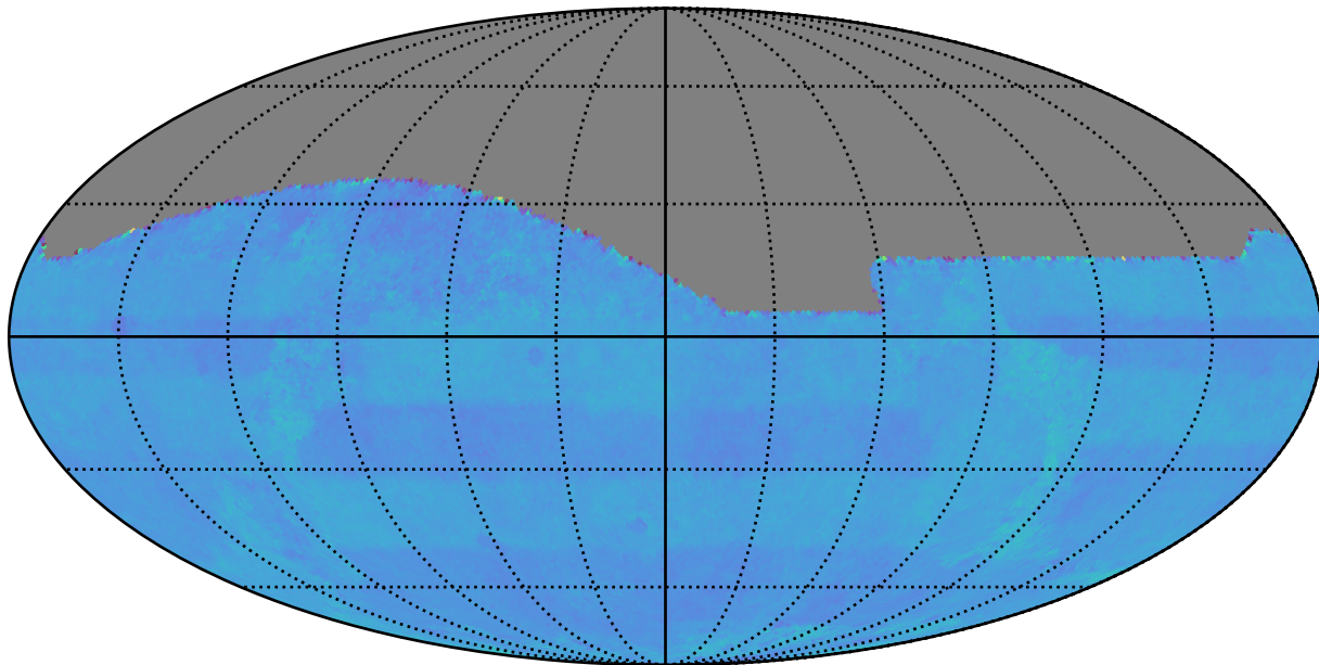
weather_cloudso10v3.4_10yrs : Normalized Proper Motion Uncert @ 24.0
