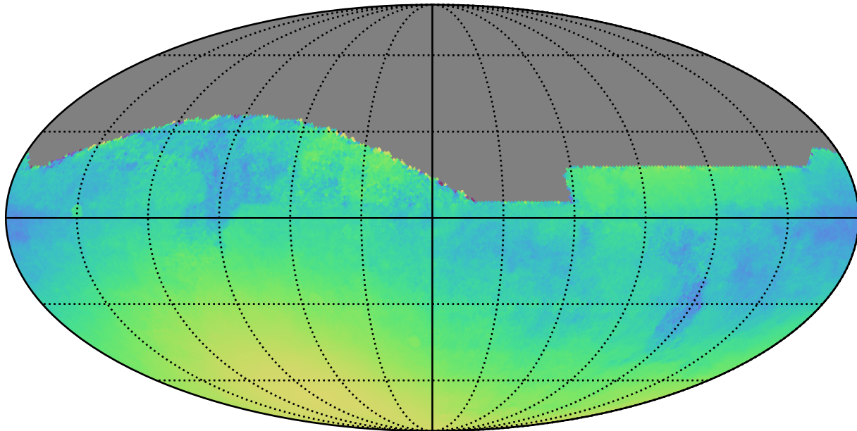
weather_cloudso10v3.4_10yrs : Normalized Parallax Uncert @ 24.0
