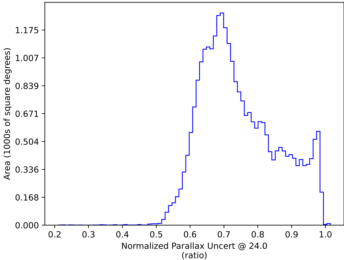
weather_cloudso10v3.4_10yrs : Normalized Parallax Uncert @ 24.0
