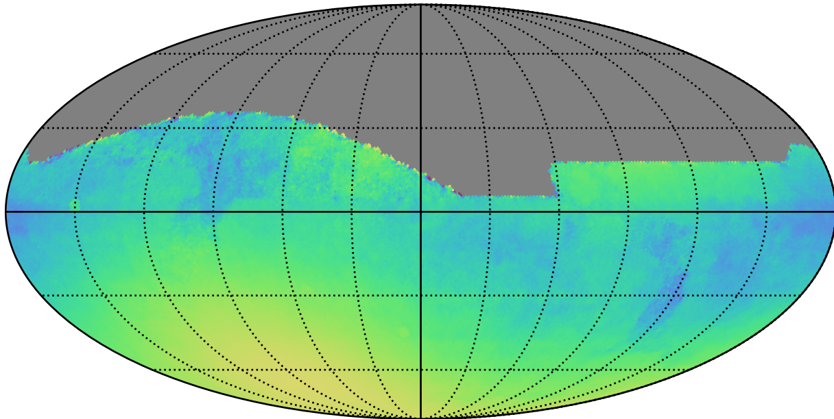
weather_cloudso10v3.4_10yrs : Normalized Parallax Uncert @ 22.4
