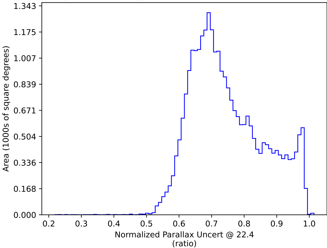
weather_cloudso10v3.4_10yrs : Normalized Parallax Uncert @ 22.4
