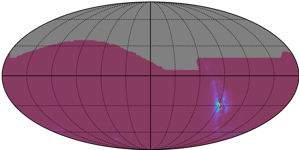
weather_cloudso10v3.4_10yrs : NlcPoints
