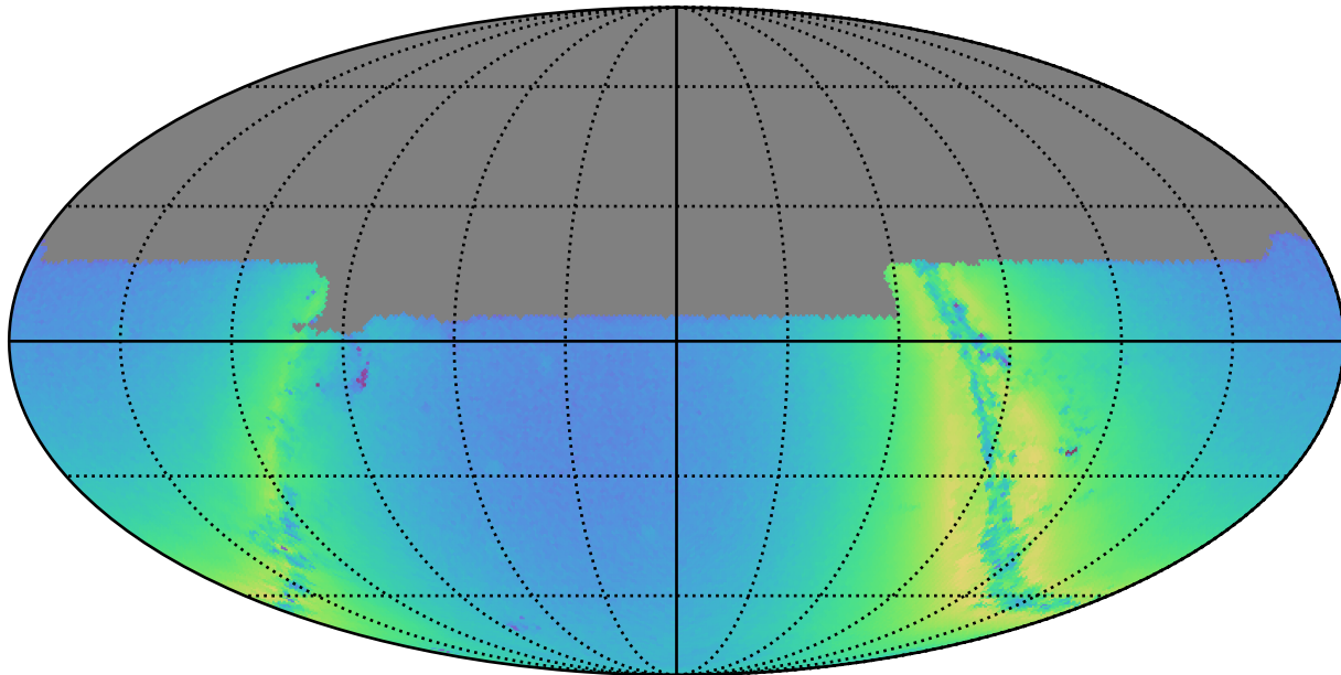
weather_cloudso10v3.4_10yrs u: N stars to Precision 0.20
