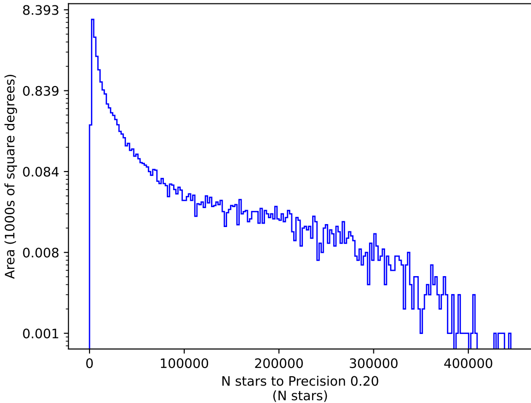
weather_cloudso10v3.4_10yrs u: N stars to Precision 0.20
