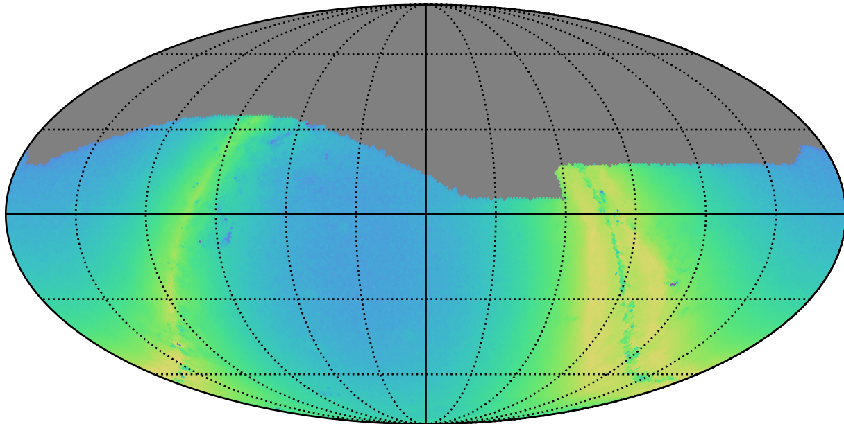
weather_cloudso10v3.4_10yrs g: N stars to Precision 0.20
