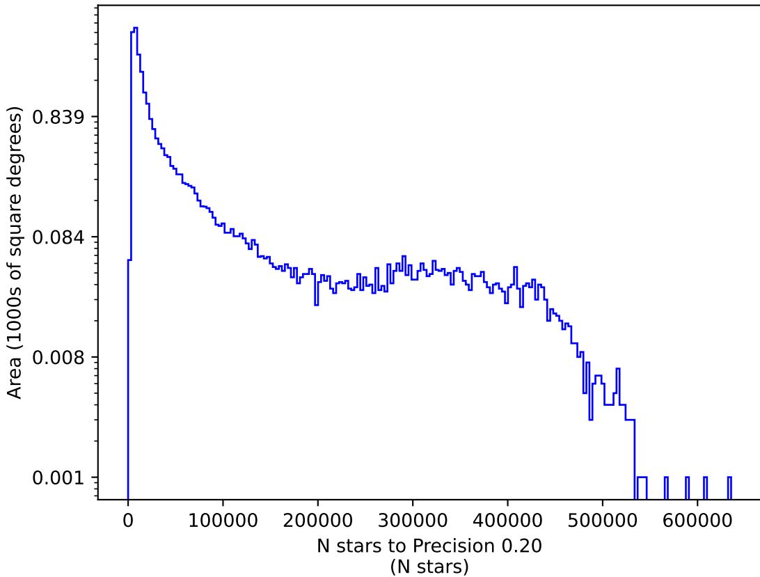
weather_cloudso10v3.4_10yrs g: N stars to Precision 0.20
