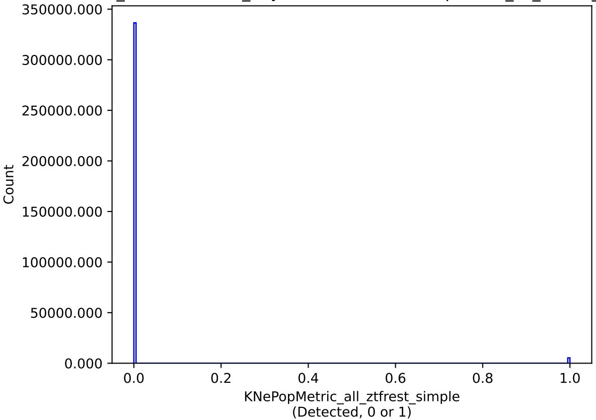
weather_cloudso10v3.4_10yrs all models: KNePopMetric_all_ztfrest_simple
