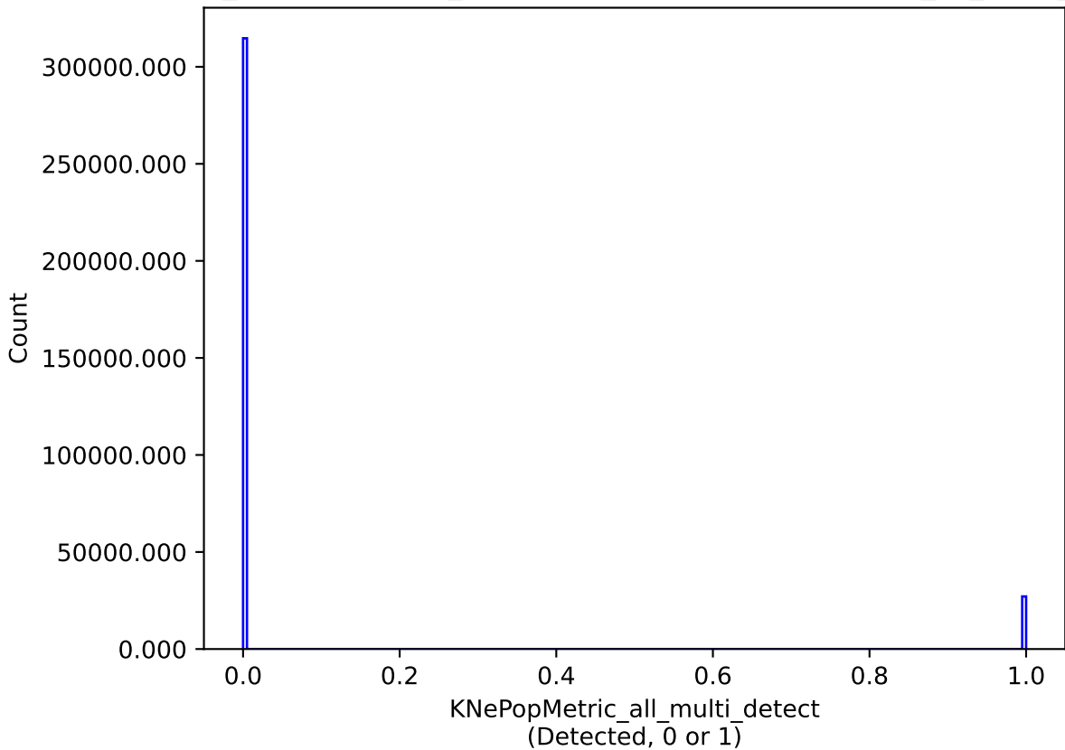
weather_cloudso10v3.4_10yrs all models: KNePopMetric_all_multi_detect
