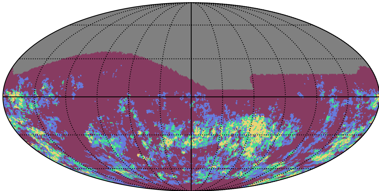
weather_cloudso10v3.4_10yrs z band: Gaps_7hr
