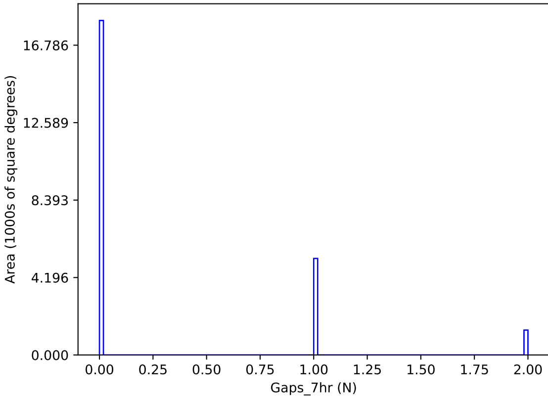
weather_cloudso10v3.4_10yrs y band: Gaps_7hr
