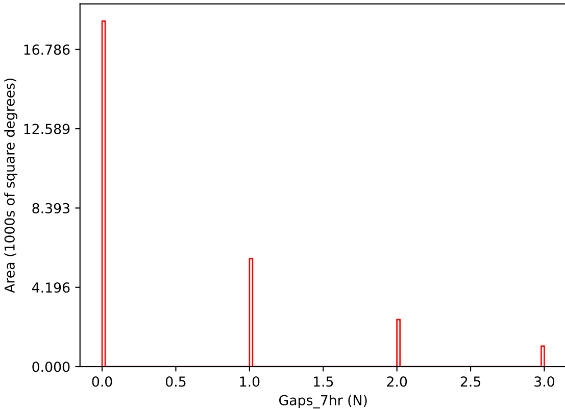
weather_cloudso10v3.4_10yrs i band: Gaps_7hr
