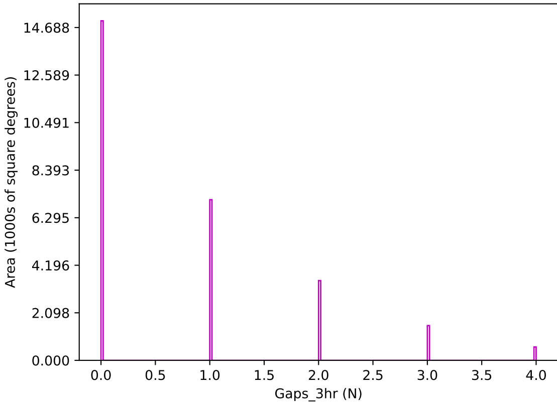
weather_cloudso10v3.4_10yrs z band: Gaps_3hr
