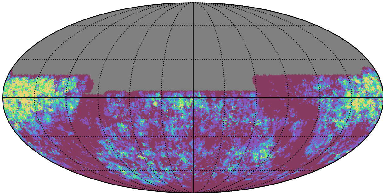
weather_cloudso10v3.4_10yrs y band: Gaps_3hr
