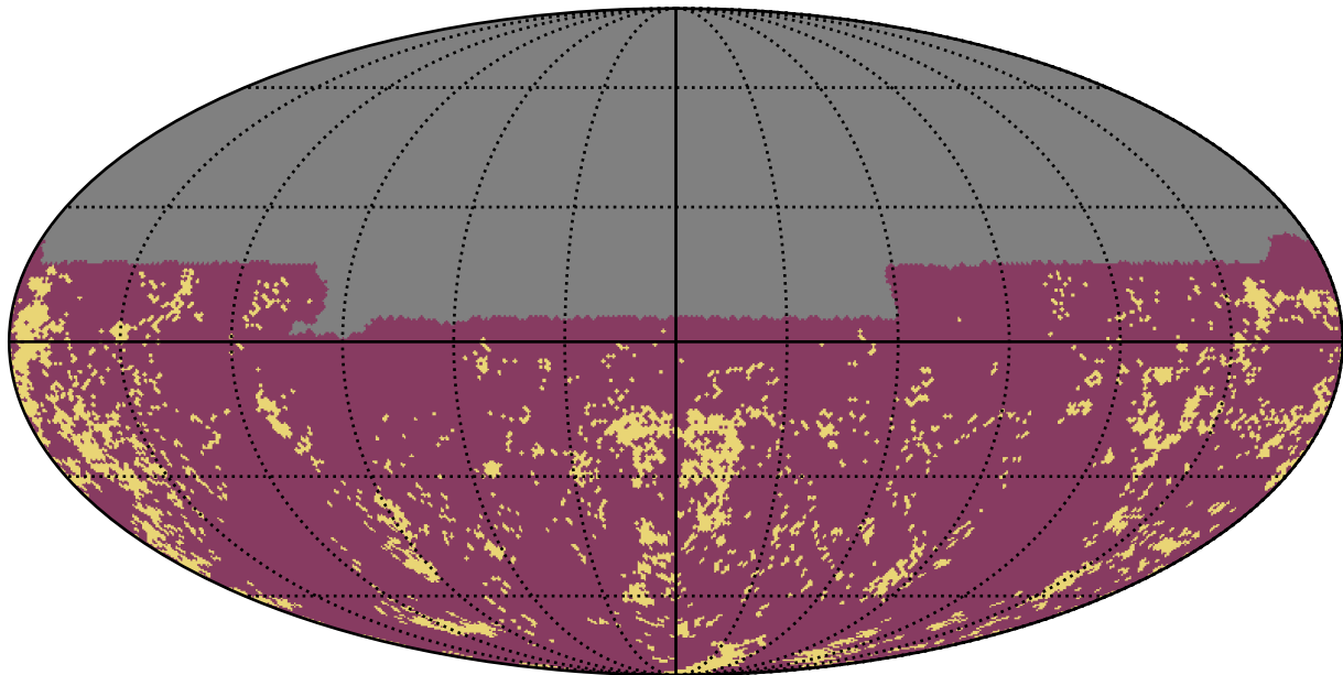
weather_cloudso10v3.4_10yrs u band: Gaps_3hr
