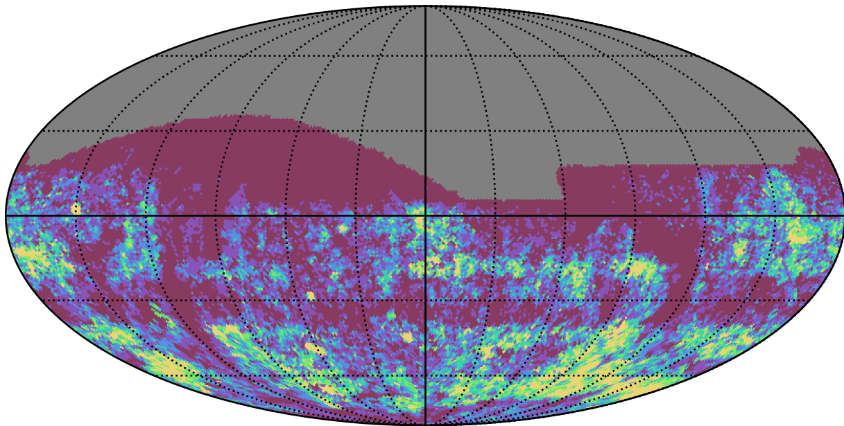
weather_cloudso10v3.4_10yrs r band: Gaps_3hr
