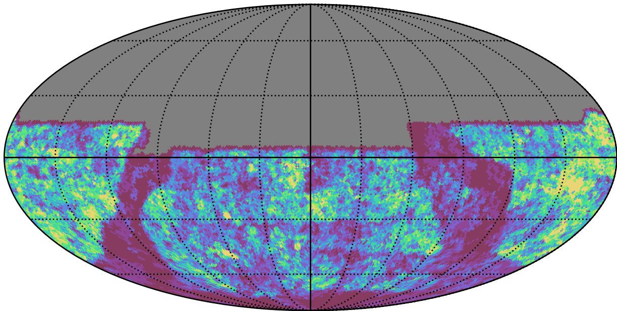
weather_cloudso10v3.4_10yrs u band: Gaps_24hr
