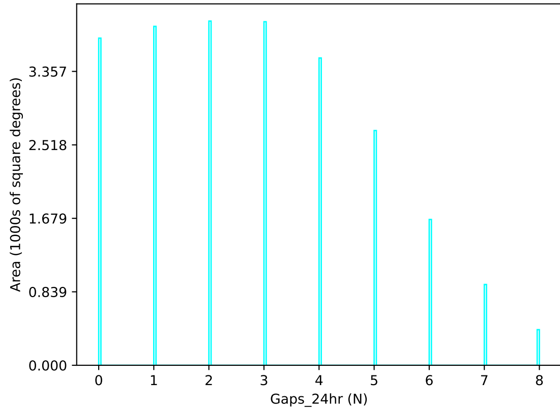
weather_cloudso10v3.4_10yrs u band: Gaps_24hr
