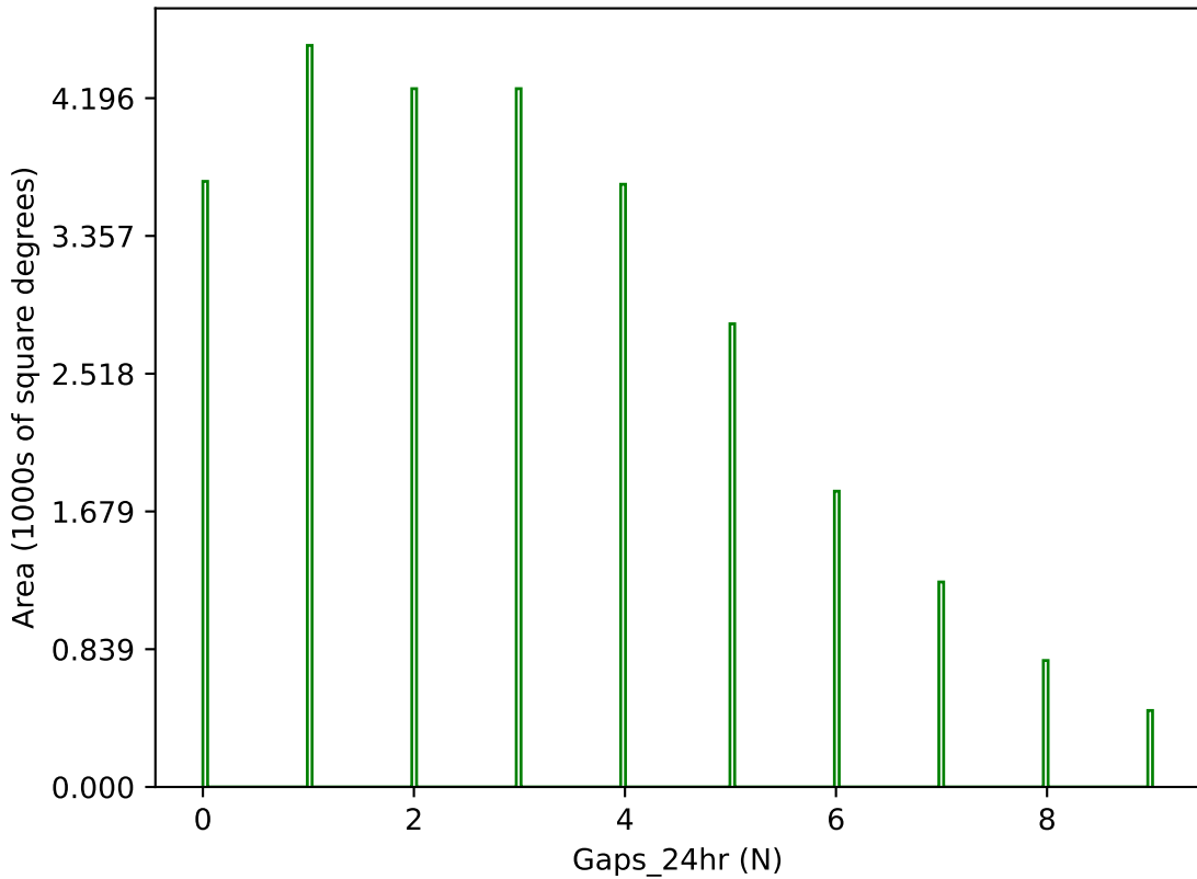
weather_cloudso10v3.4_10yrs g band: Gaps_24hr
