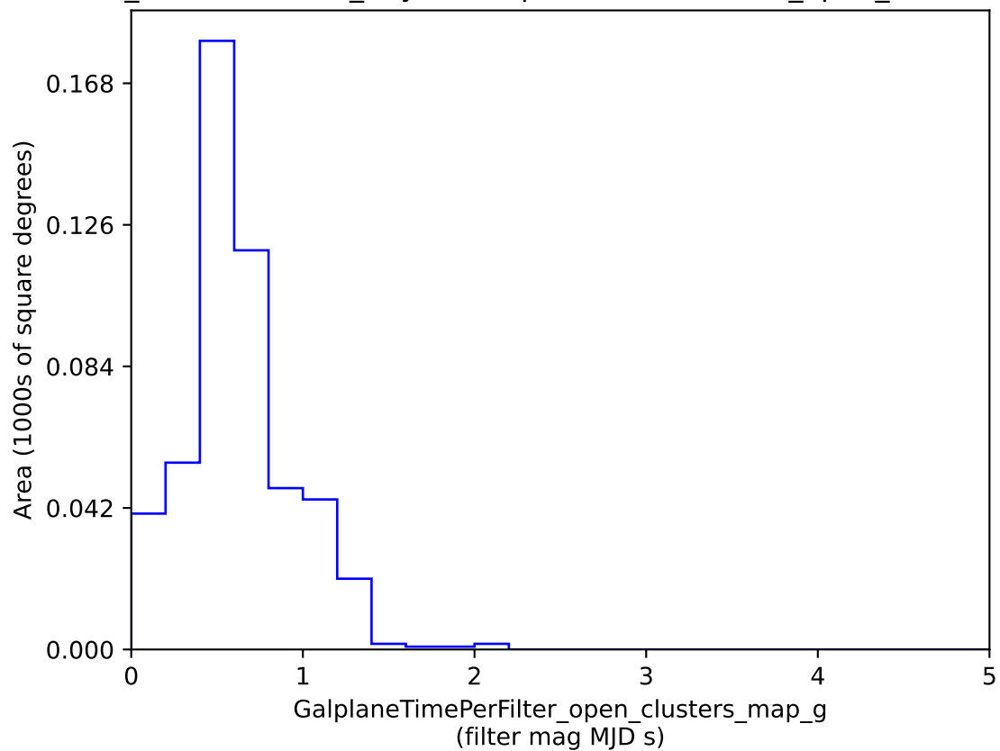
weather_cloudso10v3.4_10yrs : GalplaneTimePerFilter_open_clusters_map_g
