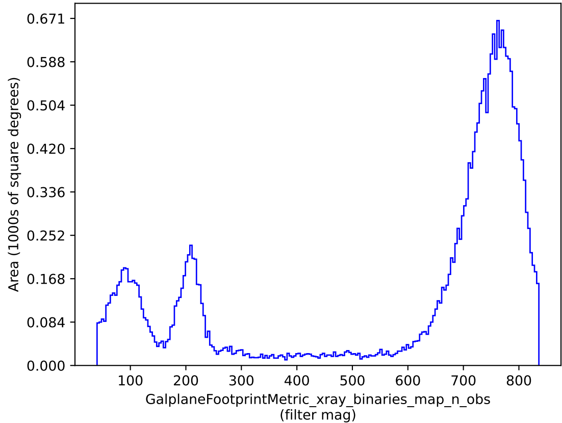
weather_cloudso10v3.4_10yrs : GalplaneFootprintMetric_xray_binaries_map_n_obs
