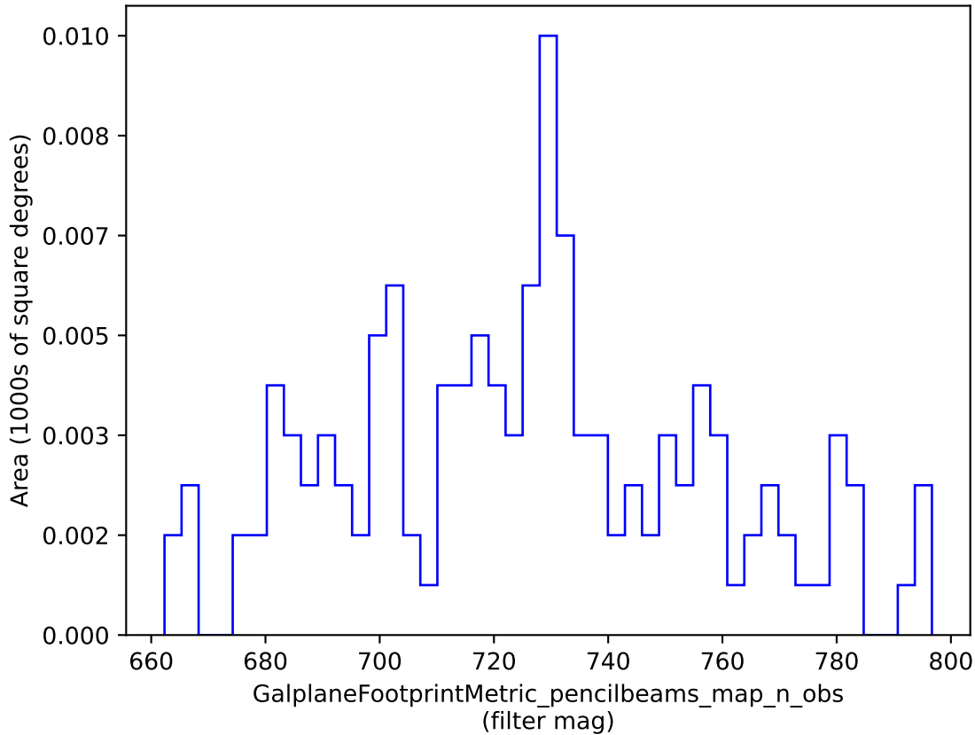
weather_cloudso10v3.4_10yrs : GalplaneFootprintMetric_pencilbeams_map_n_obs
