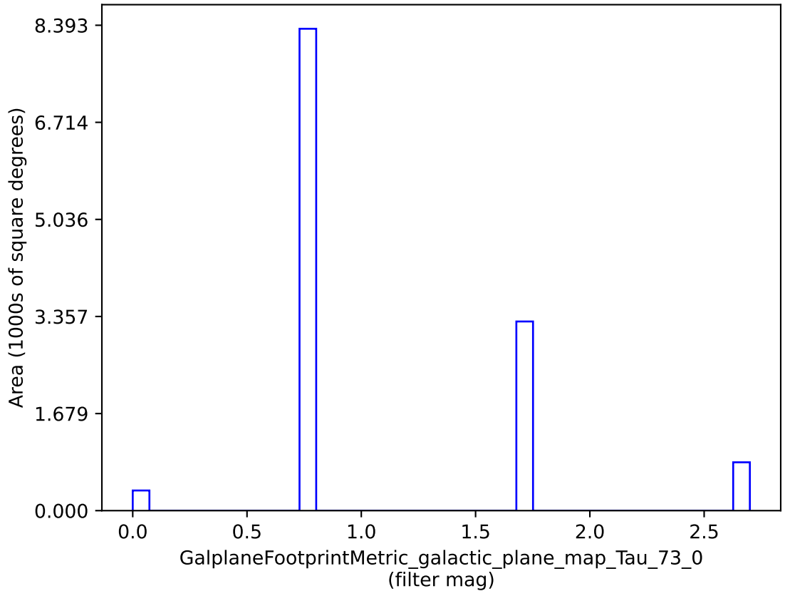
weather_cloudso10v3.4_10yrs : GalplaneFootprintMetric_galactic_plane_map_Tau_73_0
