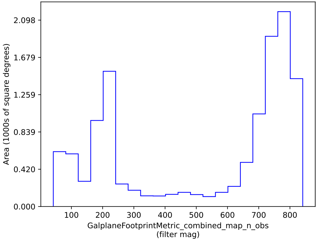
weather_cloudso10v3.4_10yrs : GalplaneFootprintMetric_combined_map_n_obs
