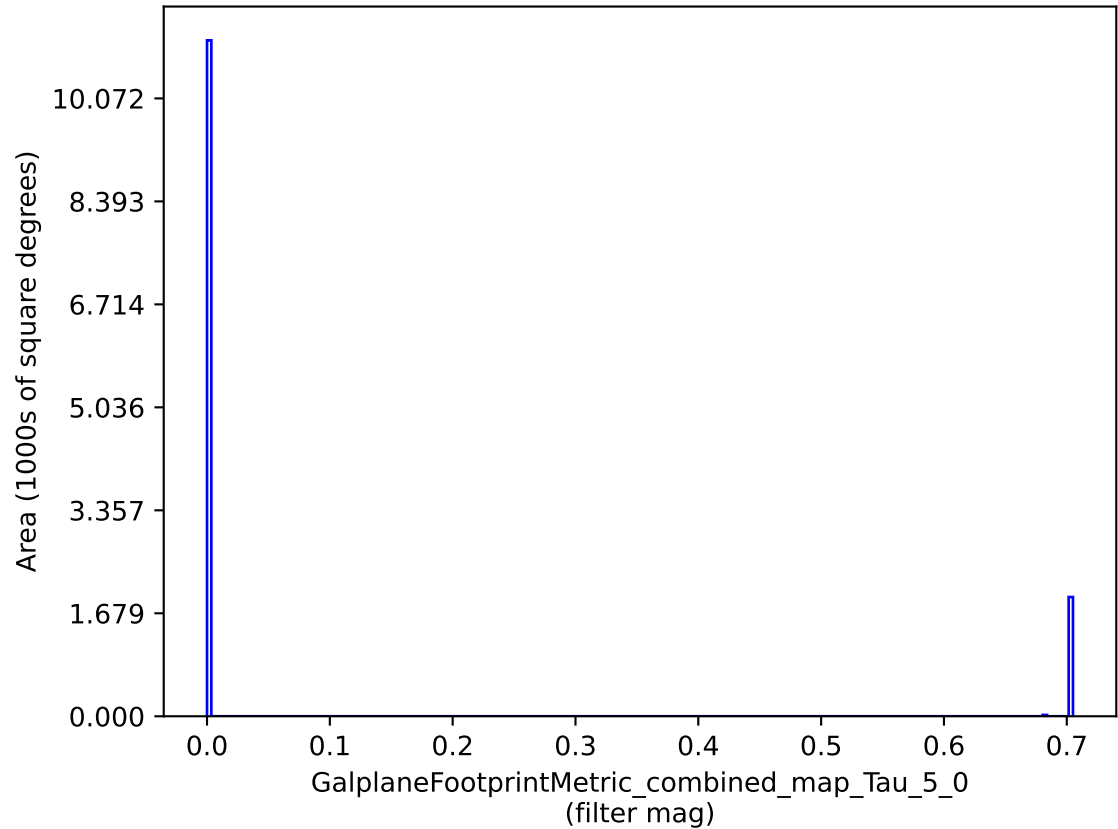
weather_cloudso10v3.4_10yrs : GalplaneFootprintMetric_combined_map_Tau_5_0
