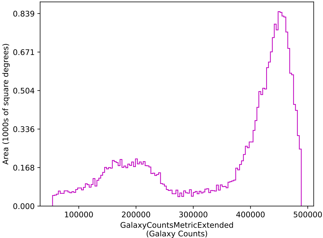
weather_cloudso10v3.4_10yrs z: GalaxyCountsMetricExtended
