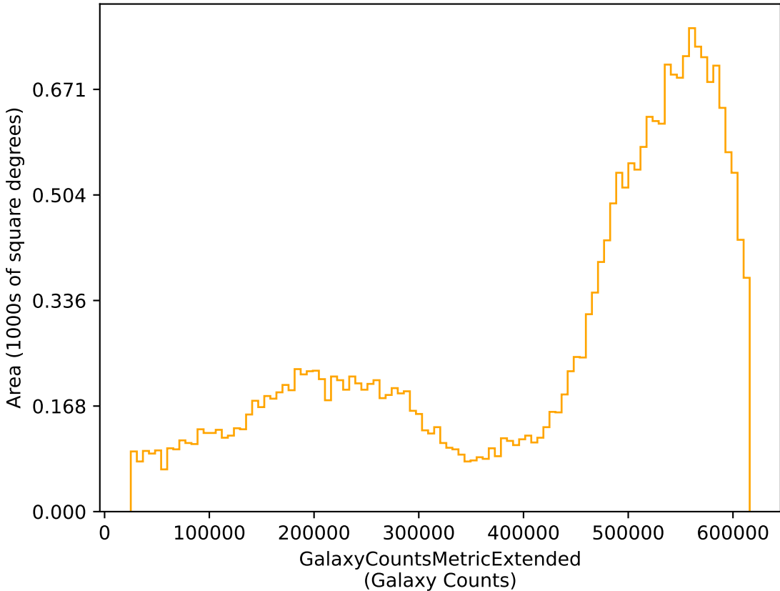
weather_cloudso10v3.4_10yrs r: GalaxyCountsMetricExtended
