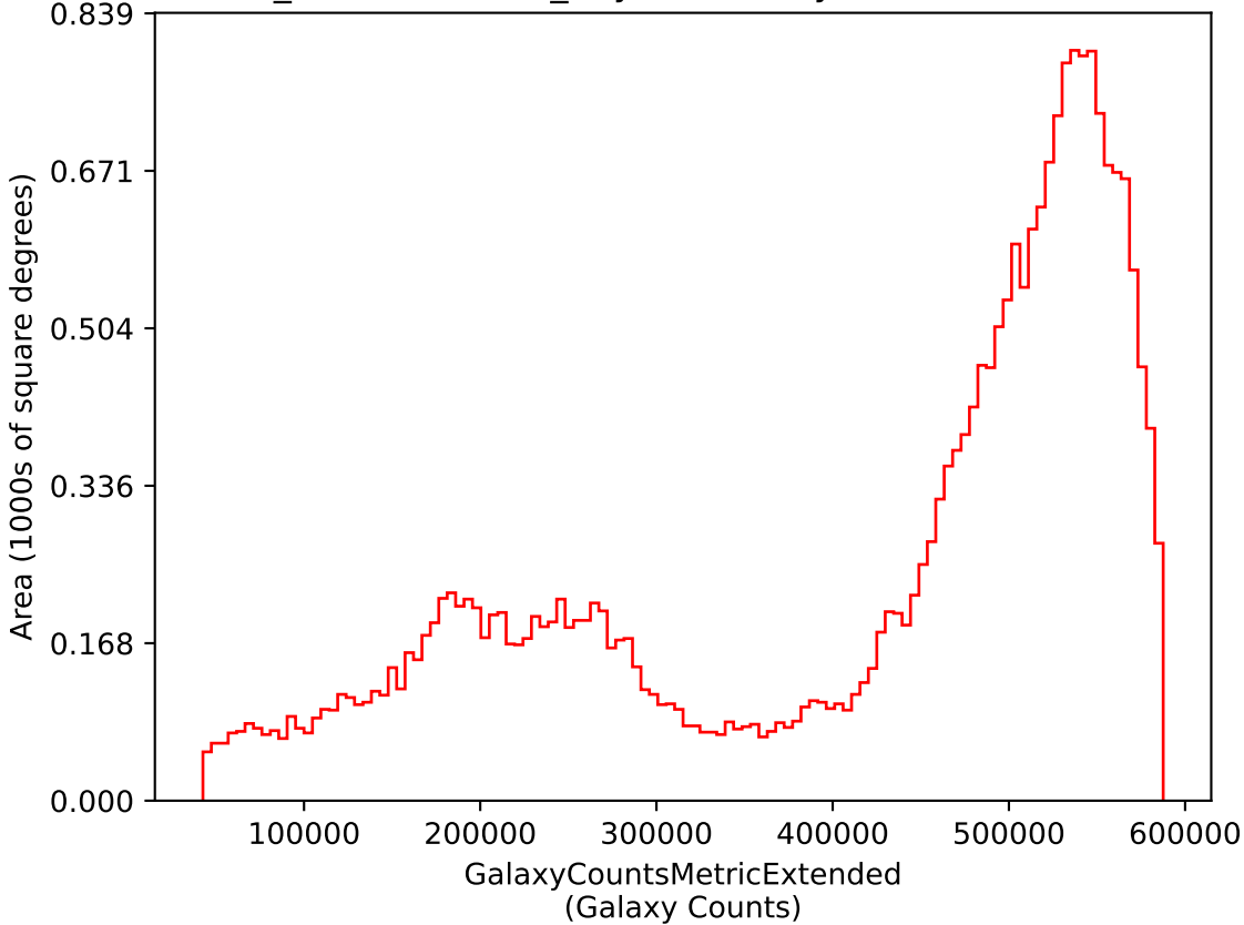
weather_cloudso10v3.4_10yrs i: GalaxyCountsMetricExtended
