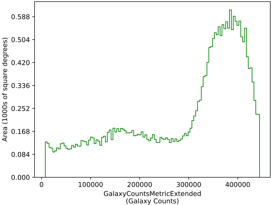
weather_cloudso10v3.4_10yrs g: GalaxyCountsMetricExtended
